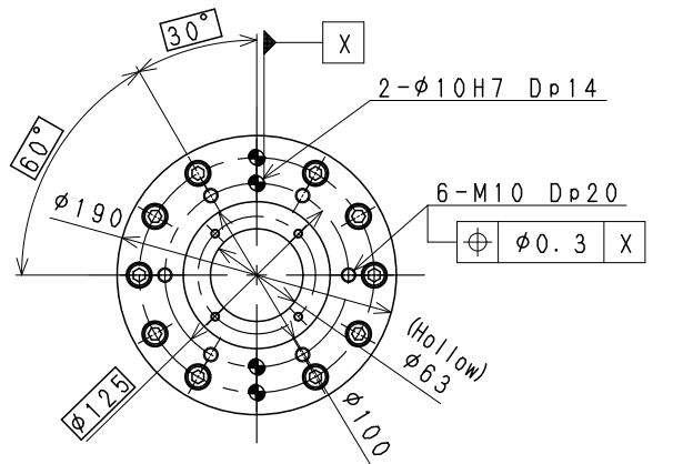
OPTION FLANGE
