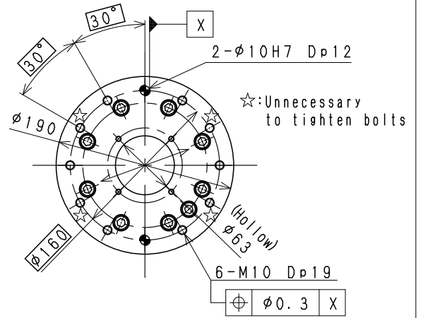
STANDARD FLANGE
